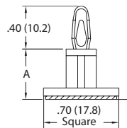
Snap Fit: .156 (4.0) Panel Thickness: .062 (1.6)
