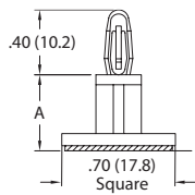
Snap Lock: .156 (4.0) Panel Thickness: .062 (1.6)
