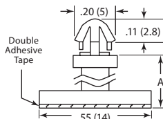
To Lock Hole: .137 (3.5) Panel Thickness: .047-.062 (1.2 - 1.6)
