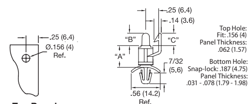
Top Board Hole Location
