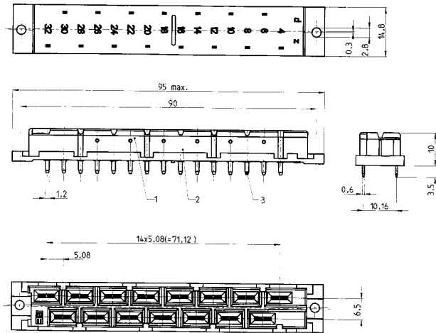
Female Connector with Solder Pin
