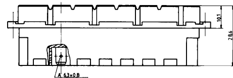
Female Connector with Faston Termination
