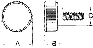
ROUND HEAD DRAWING FOR:
